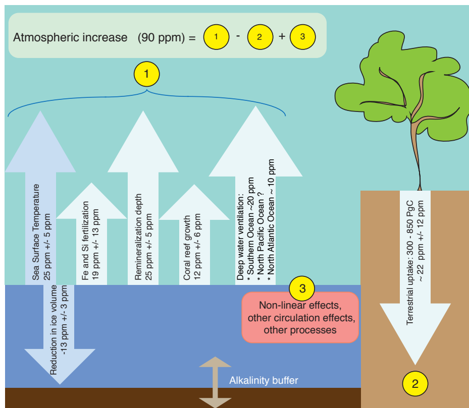
Figure 2: Best estimates of processes contributing to atmospheric CO 2 changes during the deglaciation. Dark arrows indicate high level of scientific understanding, light arrows indicate medium to low level of scientific understanding. Estimates are discussed in the text or in references in the online version of this article ( doi.org/10.22498/pages.27.2.60 ).
