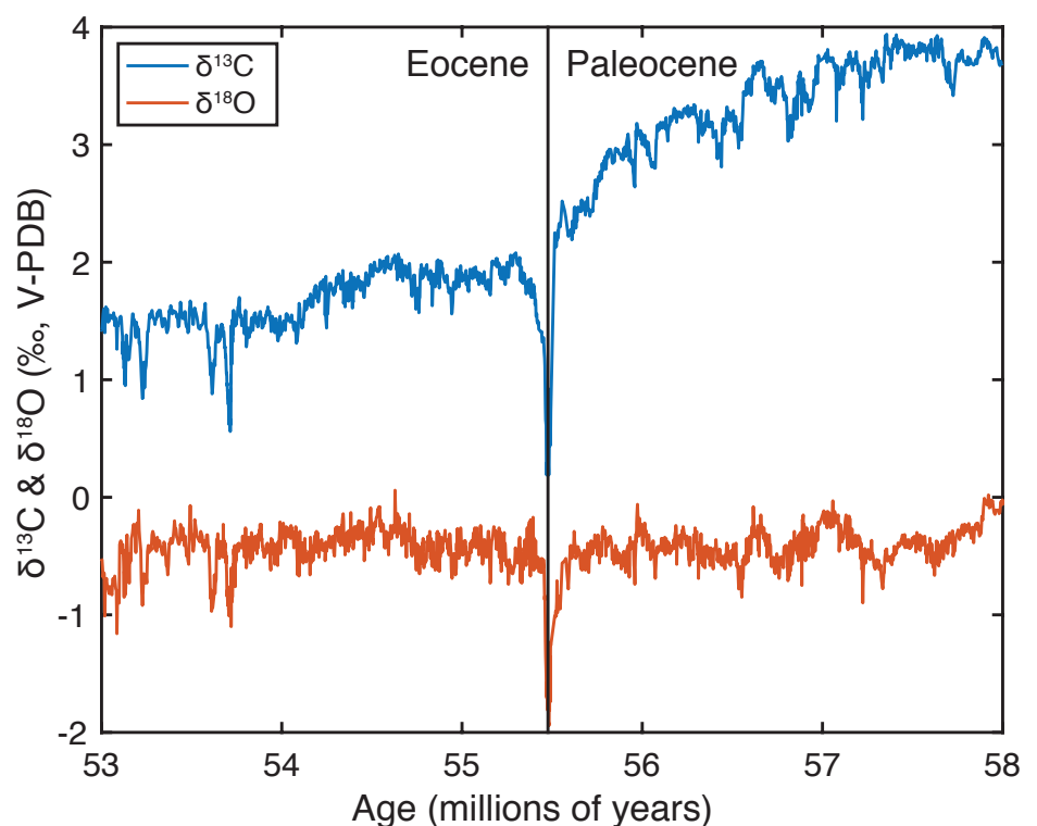
Figure 1: Bulk-sediment carbon and oxygen isotope stratigraphy of Site 1262 from the late Paleocene through the early Eocene (Zachos et al. 2010). The large negative excursions in both isotope systems at the Paleocene-Eocene boundary represents the PETM.
